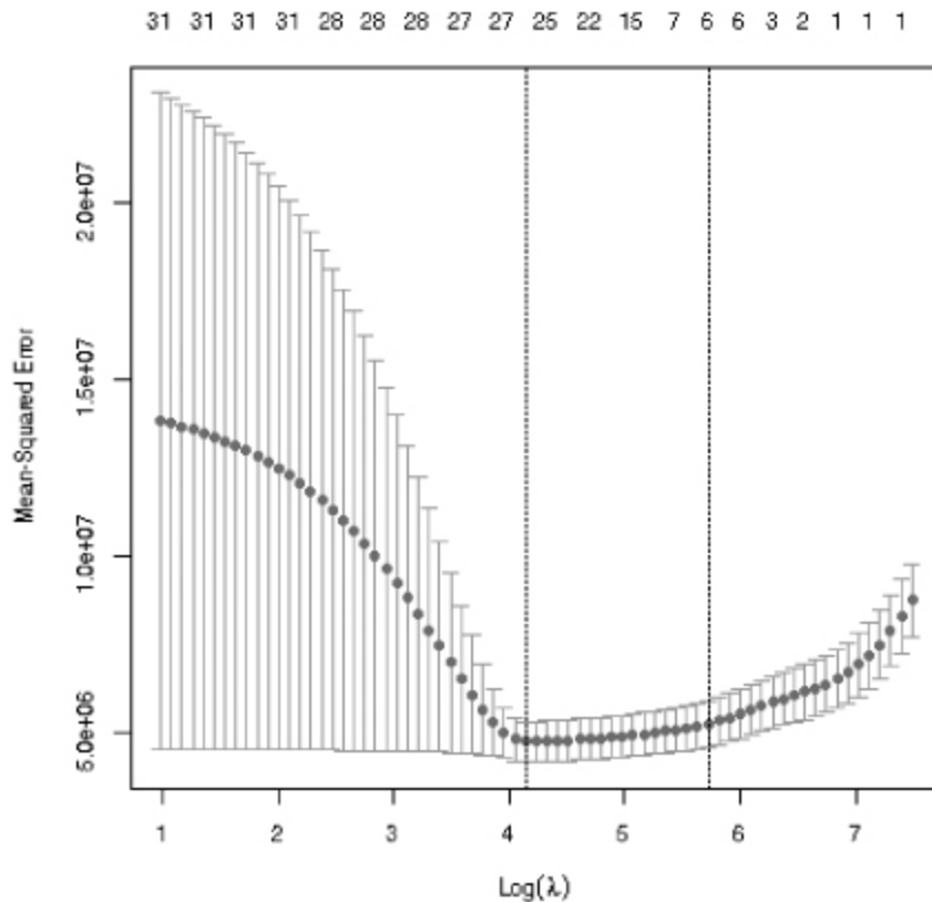
Figure 9-1: MSPE, Airbnb data
