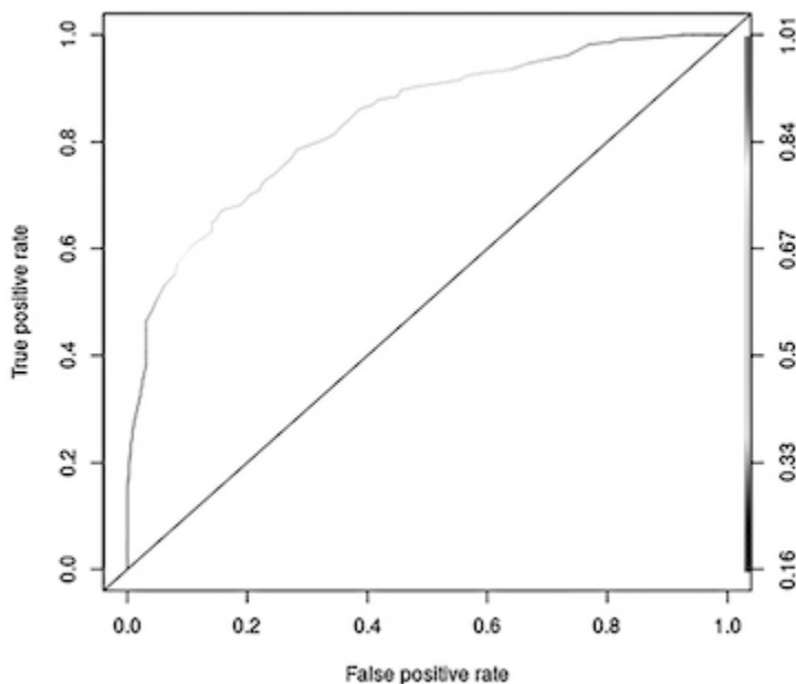
Figure 2-1: ROC, Telco Churn data
