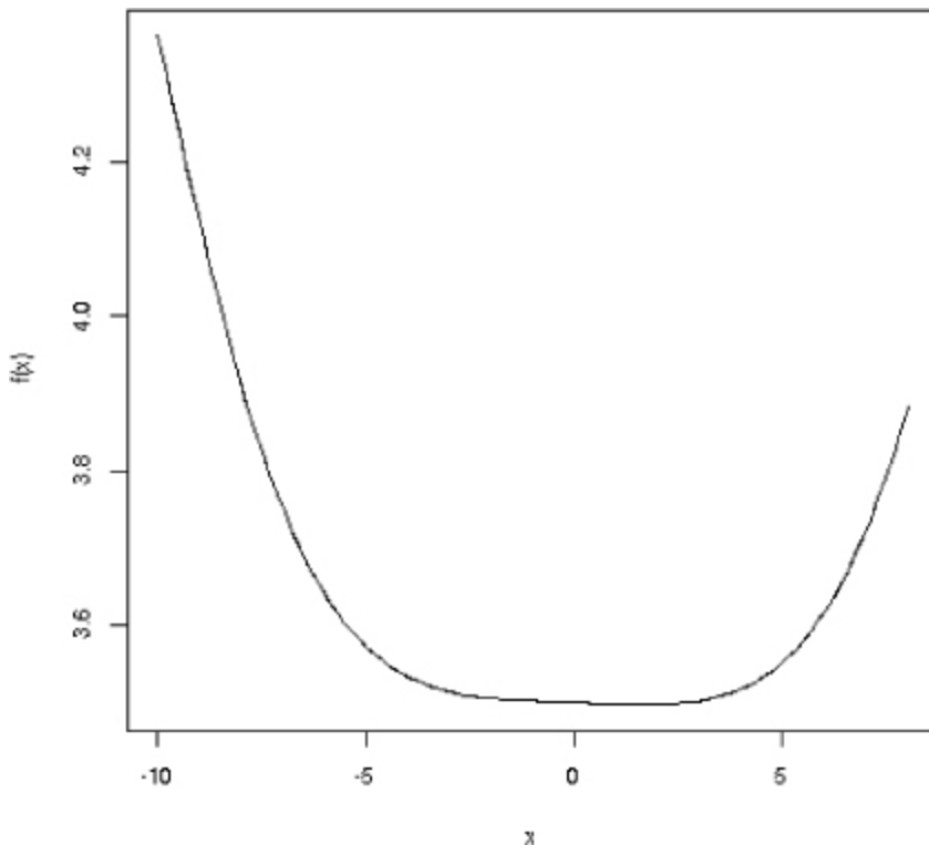
Figure 11-2: Shallow minimum region
