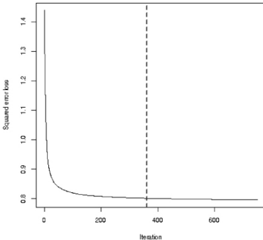
Figure 6-1: Output from gbm.perf
