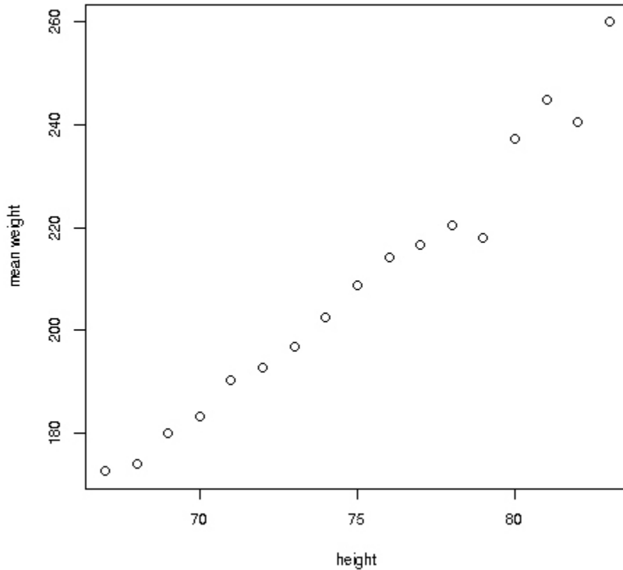
Figure 8-1: Estimated regression function, weight vs. height
