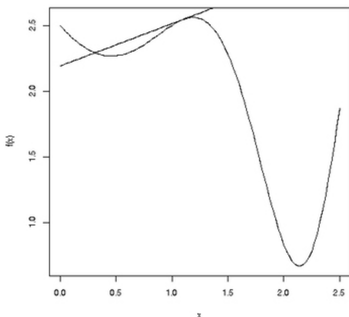
Figure 6-3: A function to be minimized, plus the tangent
