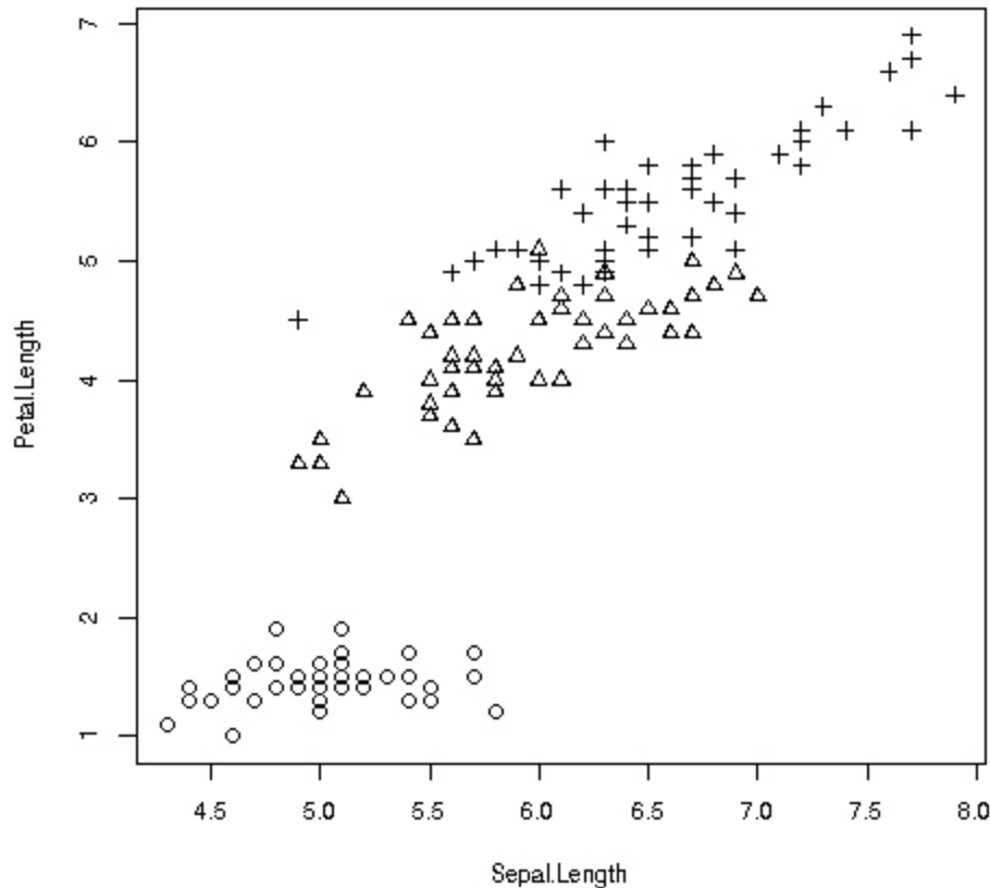
Figure 10-6: Iris data; three classes
