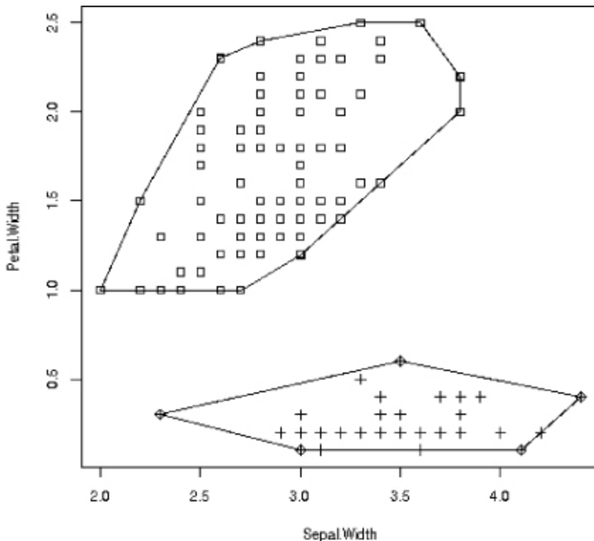
Figure 10-4: SVM convex hulls
