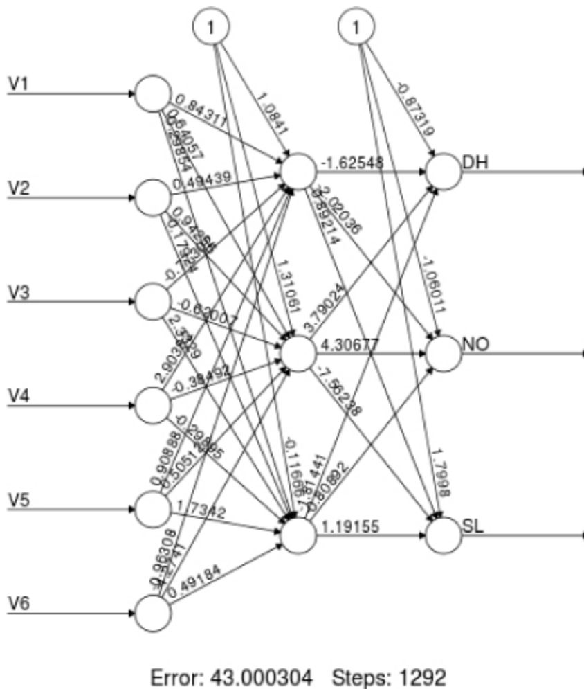
Figure 11-1: Vertebrae NN with one hidden layer
