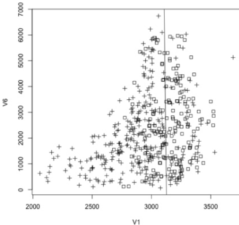
Figure 10-2: Forest cover data with a logistic boundary line
