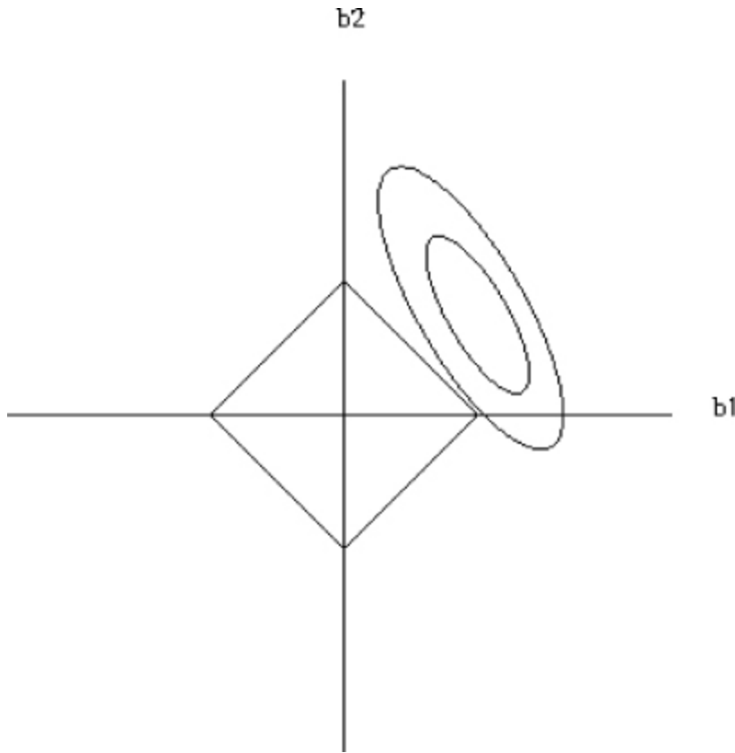
Figure 9-3: Feature subsetting nature of the LASSO
