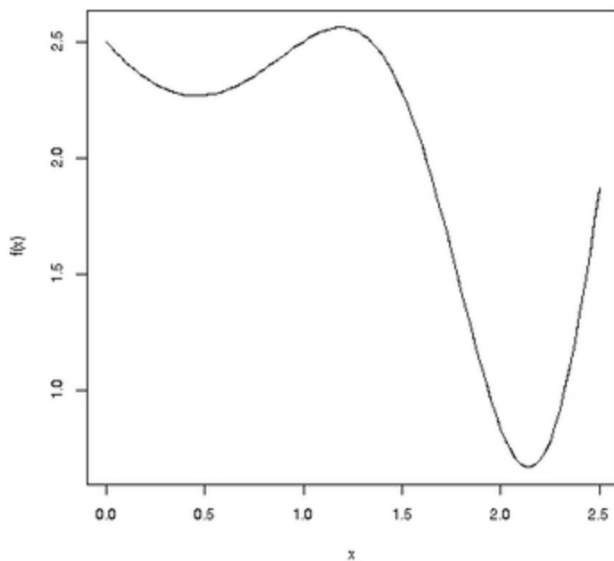
Figure 6-2: A function to be minimized
